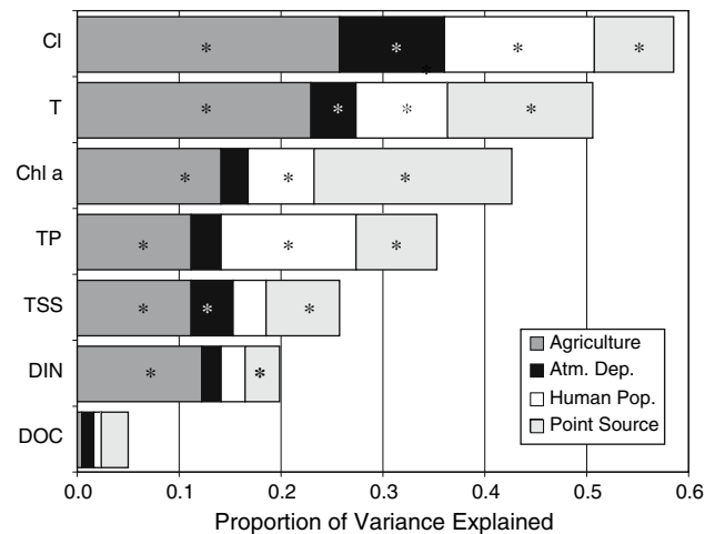
Fig. 2 Results of hierarchical partitioning of water chemistry variables on four anthropogenic stress gradients. Asterisks indicate significant predictors ( \alpha = 0.05 ) over the hierarchy of models
